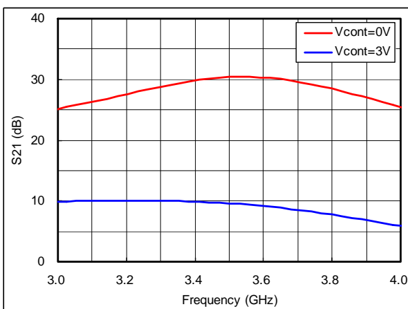
Attenuation Performance
