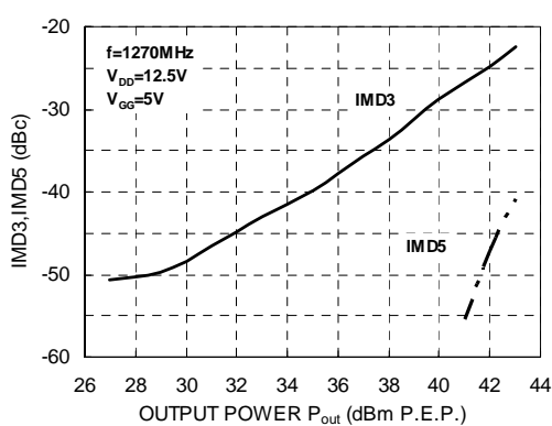
3rd,5th.INTERMODULATION DISTORTION versus OUTPUT POWER
