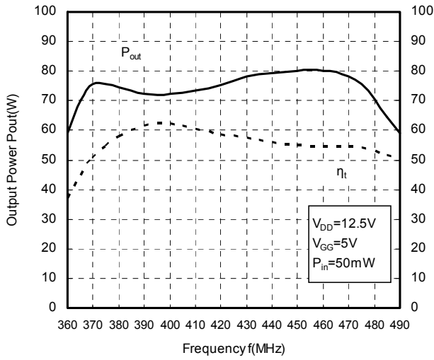
OUTPUT POWER and TOTAL EFFICIENCY, versus FREQUENCY
